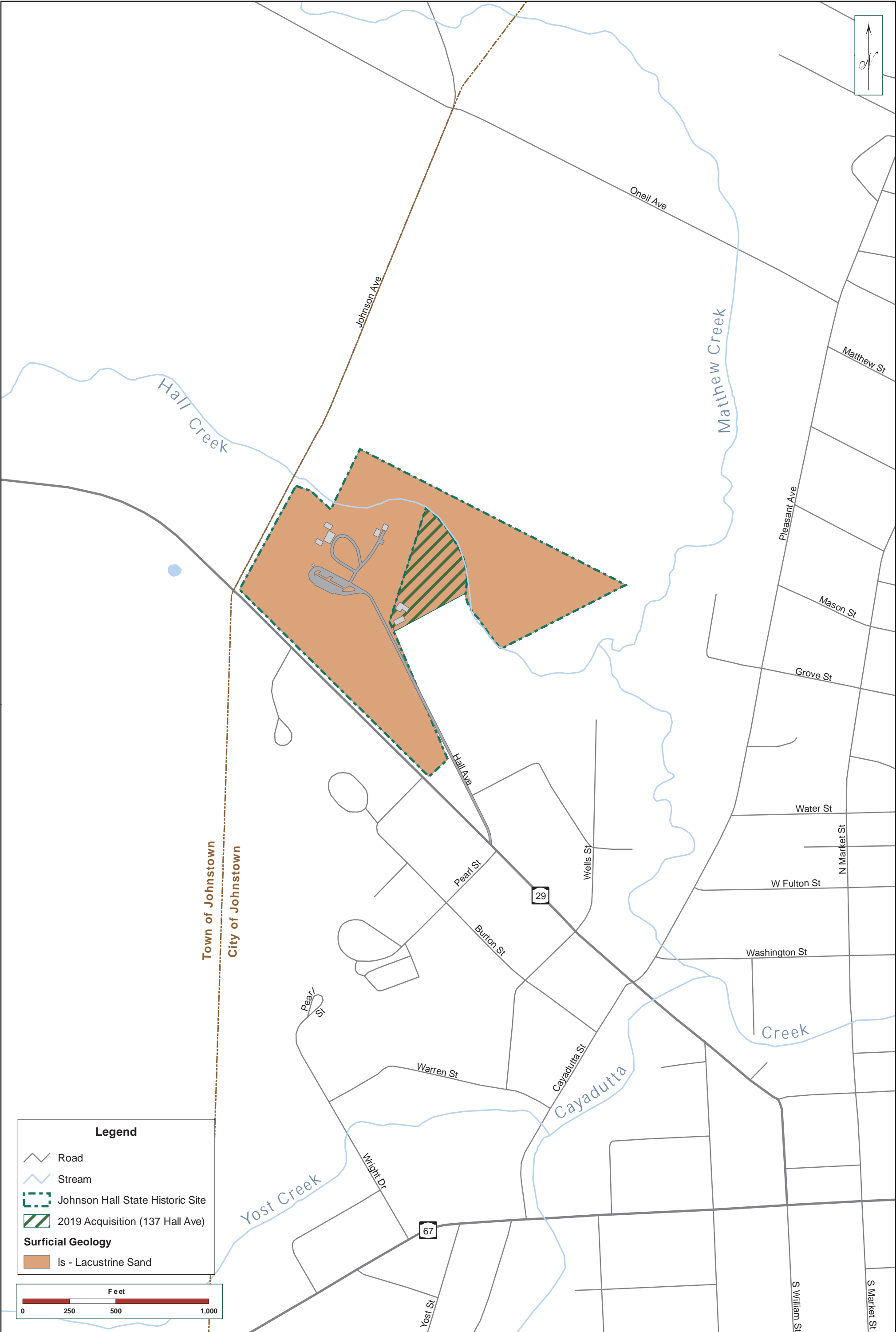
Figure 04 - Surficial Geology
