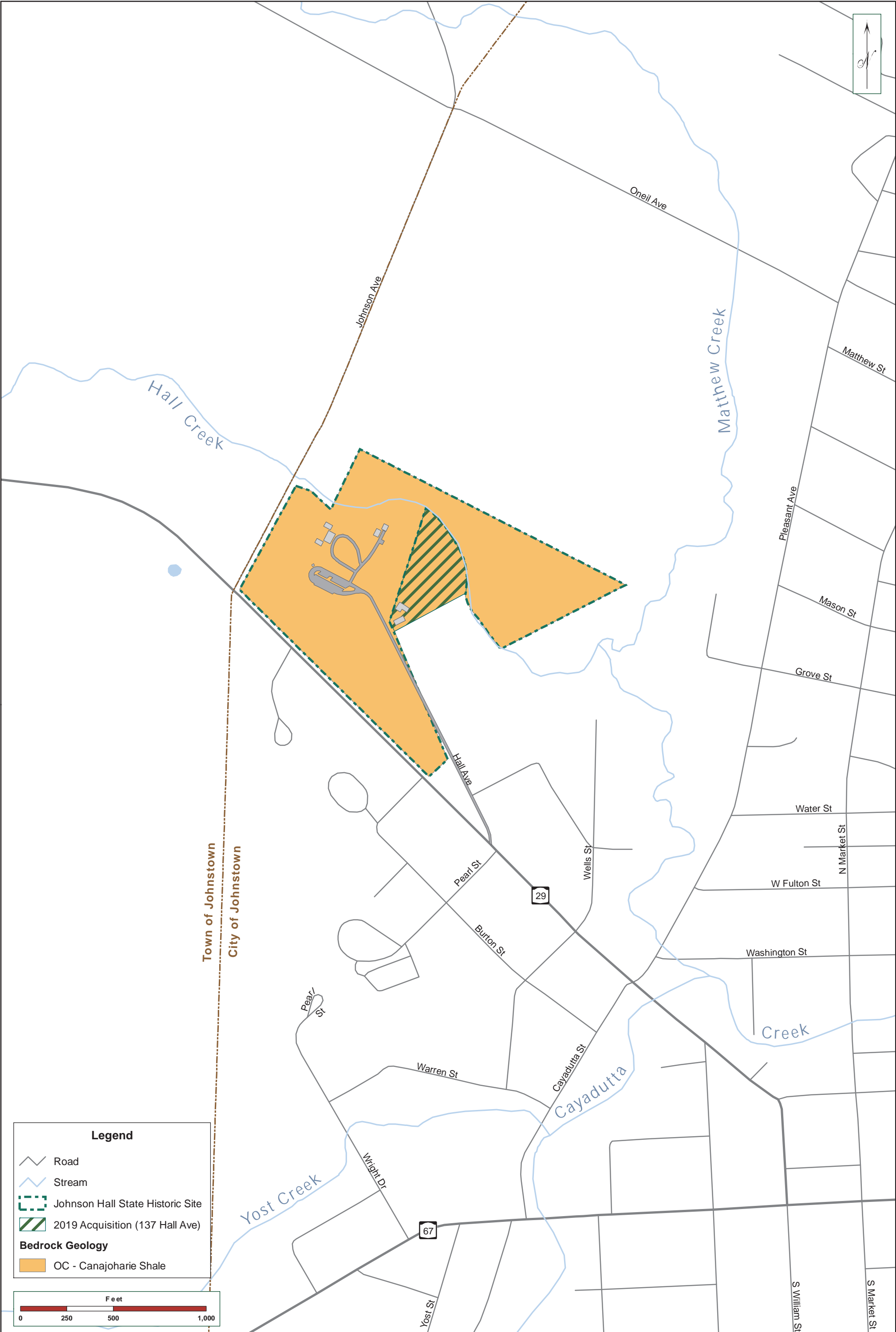
Figure 03 - Bedrock Geology
