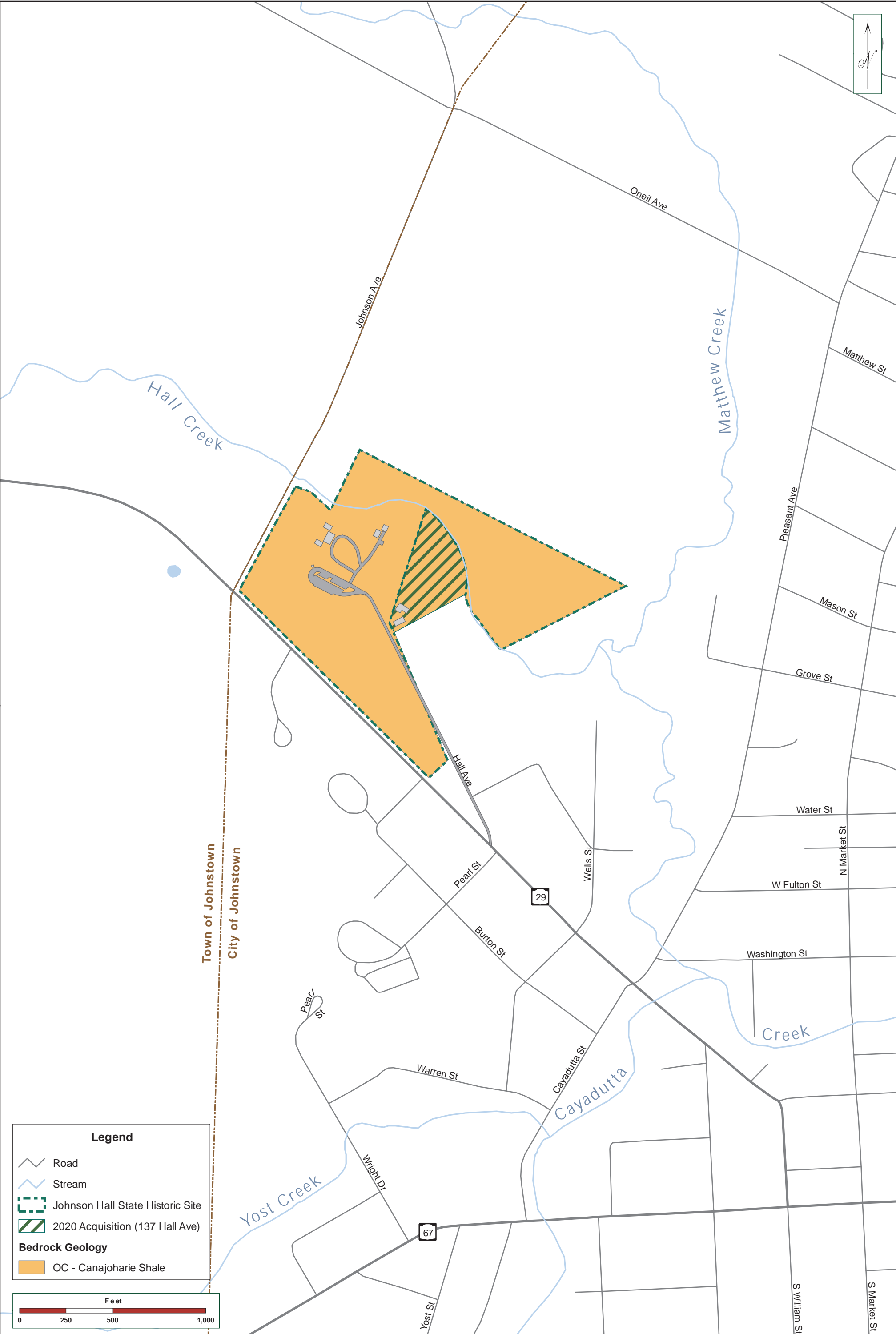
Figure 03 - Bedrock Geology
