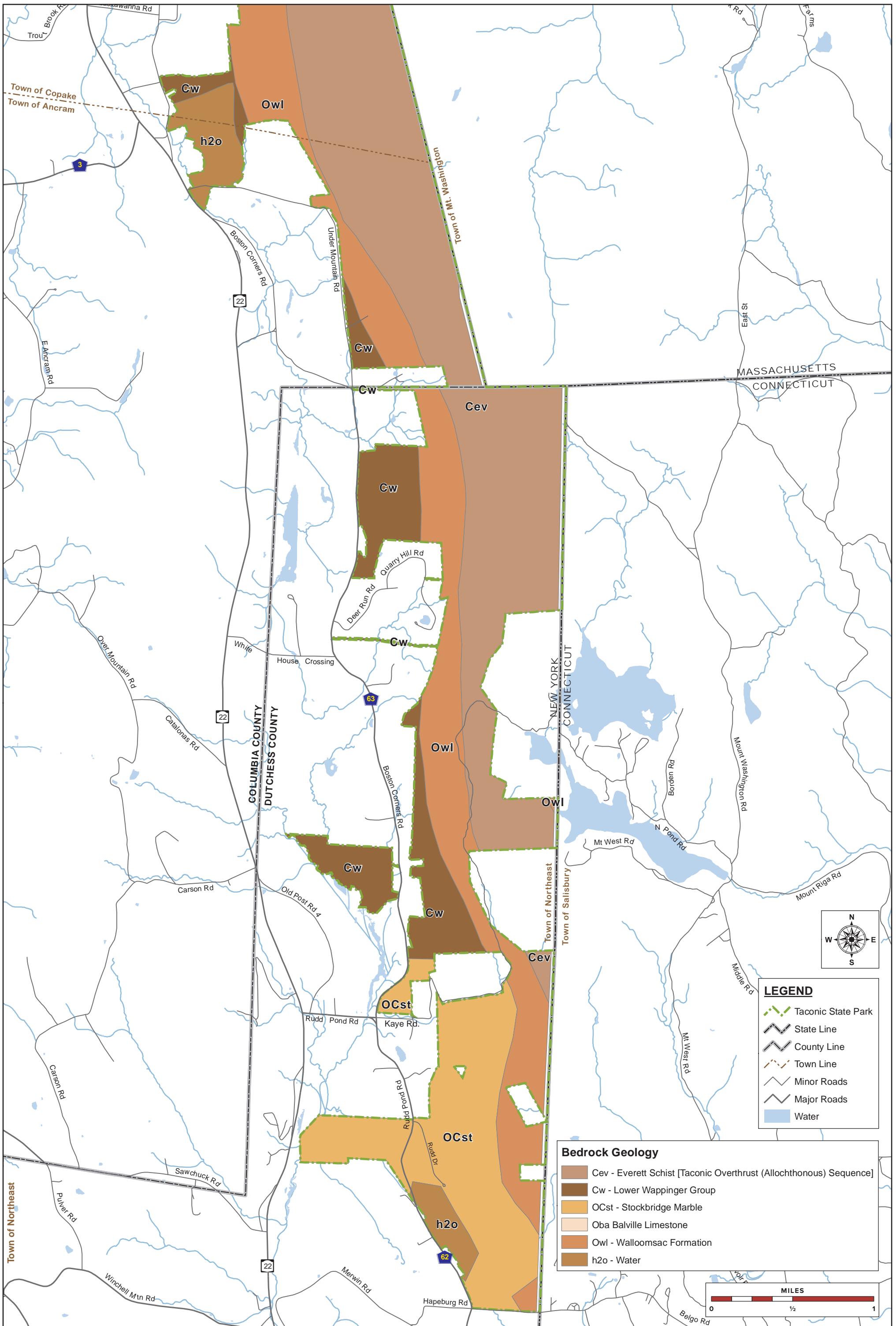
Figure 3B - BEDROCK GEOLOGY SOUTHERN SECTION
